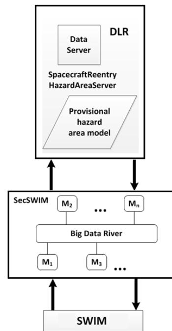
Figure 7. SecSWIM module
